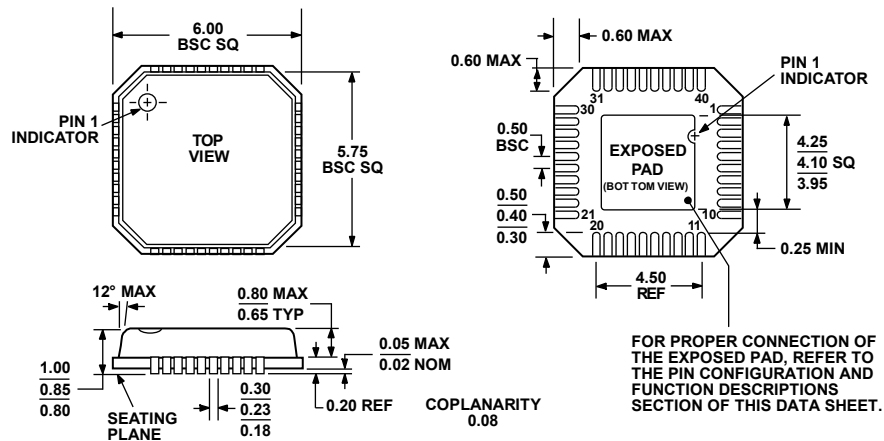
Figure 97. 40-Lead Lead Frame Chip Scale Package [LFCSP_VQ] 6 mm × 6 mm, Very Thin Quad (CP-40-1)
