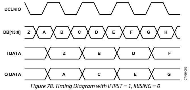
Figure 78. Timing Diagram with IFIRST = 1, IRISING = 0
