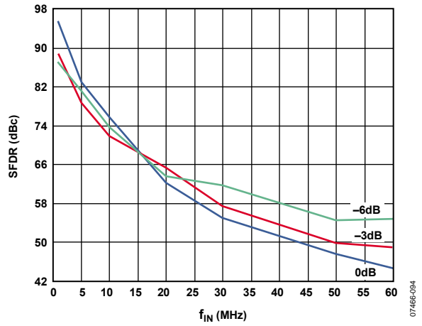
Figure 58. SFDR vs. Digital Signal Level 1.8 V
