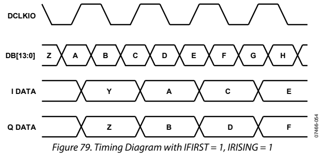
Figure 79. Timing Diagram with IFIRST = 1, IRISING = 1
