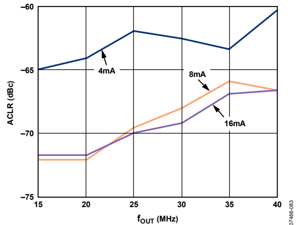
Figure 52. AD9117 2-Carrier W-CDMA Third Adjacent Channel ACLR 3.3 V
