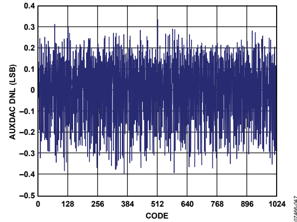
Figure 40. AUXDAC DNL
