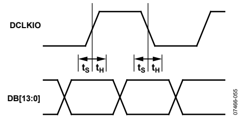
Figure 80. Set-Up and Hold Times for All Input Modes
