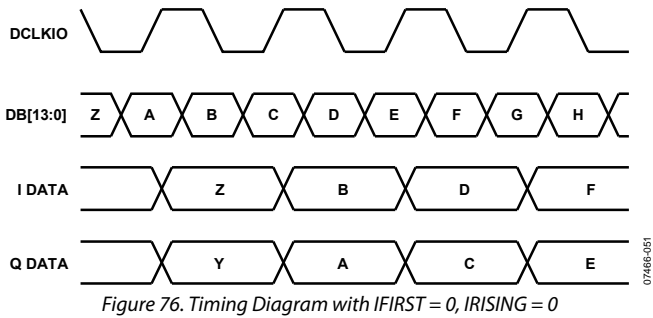
Figure 76. Timing Diagram with IFIRST = 0, IRISING = 0
