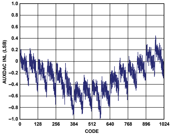
Figure 37. AUXDAC INL
