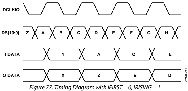
Figure 77. Timing Diagram with IFIRST = 0, IRISING = 1
